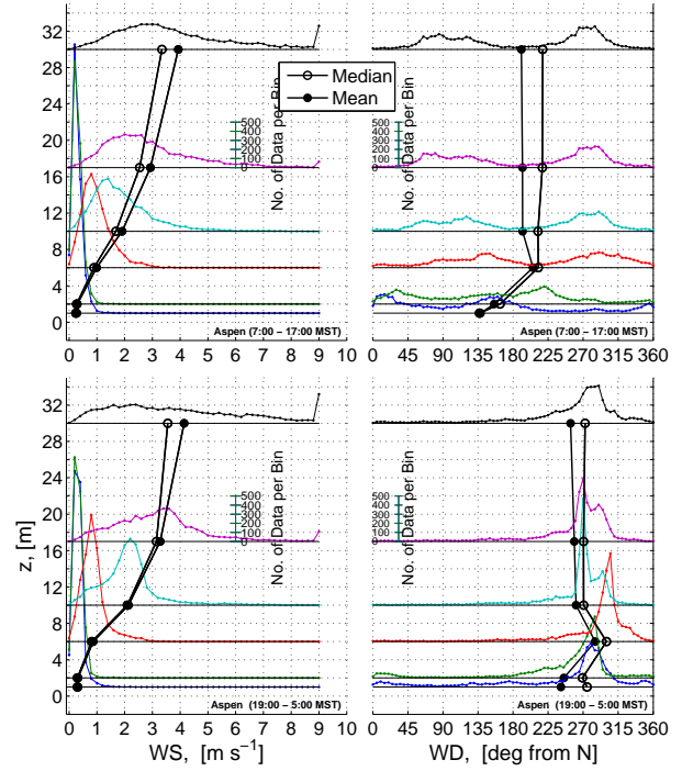
Figure 11: Frequency distributions of (a) wind speed WS, and (b) wind direction WD at different levels on the Aspen tower for daytime (top panels) and nighttime (lower panels).
