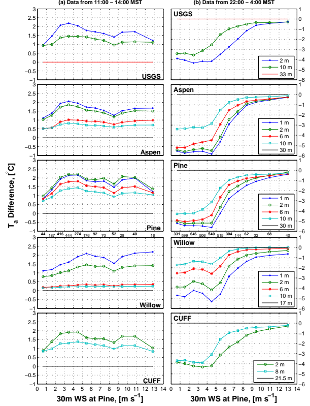
Figure 2: The vertical gradient of air temperature T_a measured at each tower binned by the 30m-WS at the Pine tower (the lower levels are subtracted from the highest measurement level). Note that the y-axis range of the left and right panels differ. The number of 5-min data values for each bin is shown between the panels for Willow and Pine (the number of possible 5-min samples is 2196 for the daytime data and 4392 for the nighttime).
