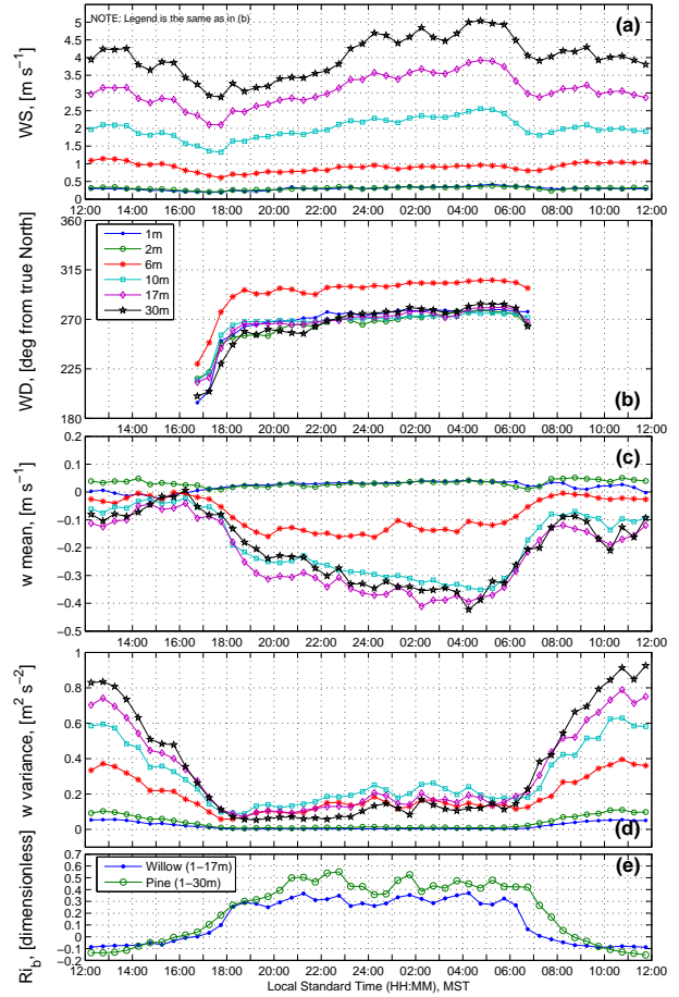
Figure 13: Half-hourly binned mean measurements at the Aspen Tower for (a) wind speed WS, (b) wind direction WD, (c) 5-min vertical wind (mean), (d) 5-min vertical wind variance, and (e) bulk Richardson number.
