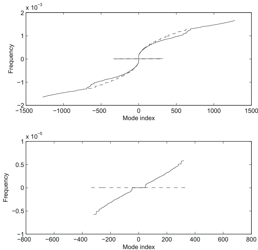
Fig. 11. Normal mode frequencies on the f -sphere. The upper panel is like the upper panel in Fig. 10 but for a scheme that constructs edge tangential velocities by projection of nearby normal velocities. The lower panel shows the same data but with a much expanded frequency scale to make clear the non-zero frequencies of the geostrophic modes.
