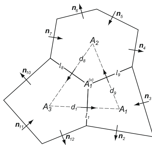
Fig. 2. Schematic showing the geometrical information needed to define a C-grid scheme on an arbitrary polygonal grid: primal edges are shown by continuous lines and dual edges by dashed lines; l_e is the length of primal edge e ; d_e is the length of dual edge e ; A_i is the area of primal cell i ; A_v^{(v)} is the area of dual cell v ; n_e is the unit normal at edge e indicating the direction corresponding to positive u_e .
