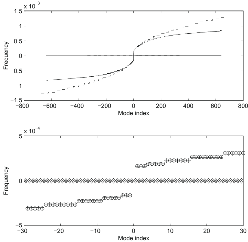
Fig. 8. Normal mode frequencies on the f -sphere. The upper panel shows the full spectrum of frequencies resolved on a hexagonal geodesic grid with 2562 degrees of freedom using the proposed scheme to compute the Coriolis terms (continuous curves) along with the exact normal mode frequencies given by (47) for n \leq 25 (dashed curves). The lower panel shows a subset of frequencies with smallest indices: circles and diamonds indicate exact normal mode frequencies; plus and cross symbols indicate numerical normal mode frequencies.
