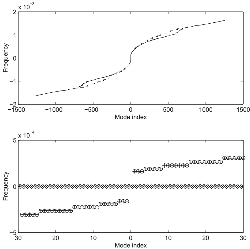
Fig. 10. Normal mode frequencies on the f -sphere. The upper panel shows the full spectrum of frequencies resolved on a triangular geodesic grid with 3200 degrees of freedom using the proposed scheme to compute the Coriolis terms (continuous curves) along with the exact normal mode frequencies given by (47) for n \leq 25 (dashed curves). The lower panel shows a subset of frequencies with smallest indices: circles and diamonds indicate exact normal mode frequencies; plus and cross symbols indicate numerical normal mode frequencies.
