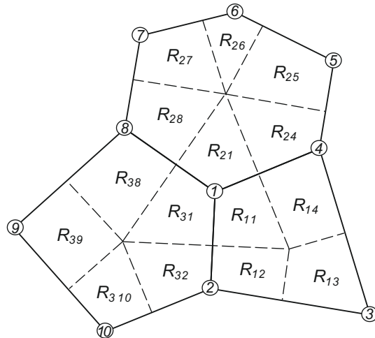
Fig. 4. Schematic showing the locations of the weights R_{iv} that define the vertex divergence in terms of the cell divergence.
