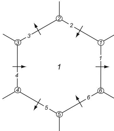
Fig. 7. Schematic showing the cell, edge and vertex numbering, and unit normal vectors at cell edges, for part of a regular hexagonal grid.
