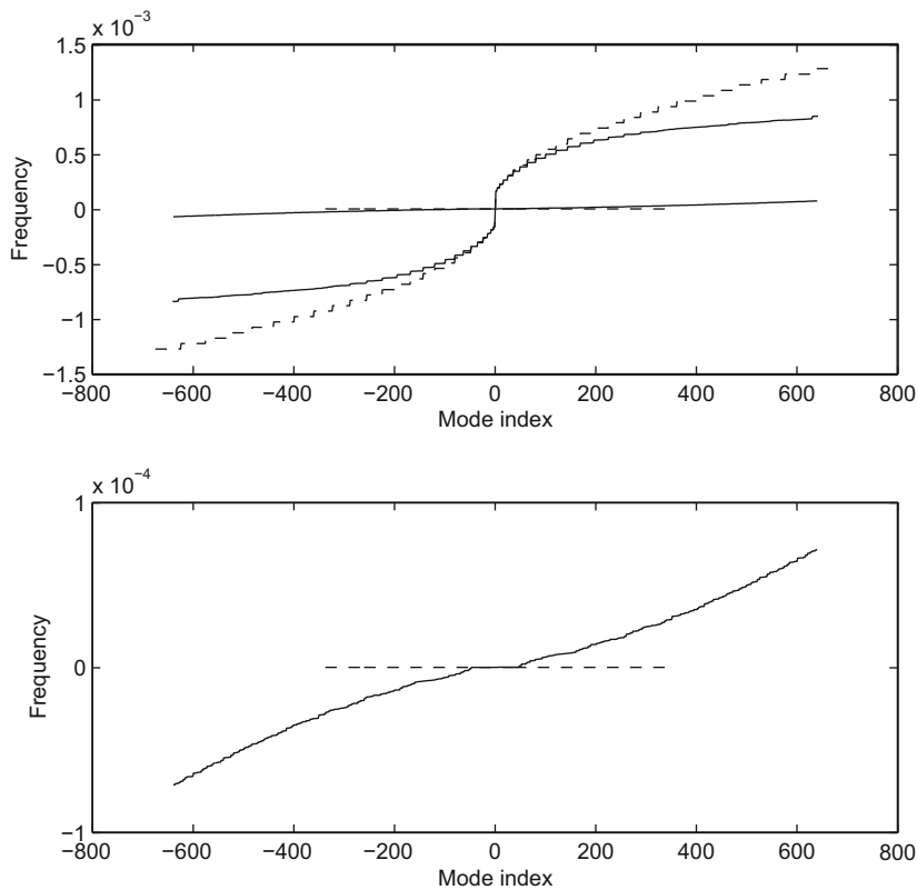
Fig. 9. Normal mode frequencies on the f -sphere. The upper panel is like the upper panel in Fig. 8 but for a scheme that reduces to the scheme used by [16] on a plane regular hexagonal grid. The lower panel shows the same data but with a much expanded frequency scale to make clear the non-zero frequencies of the geostrophic modes.
