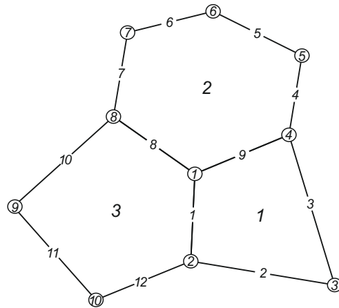
Fig. 1. Schematic showing part of an arbitrary polygonal grid. Cells, edges and vertices are each numbered with unique but otherwise arbitrary indices; this numbering will be used to give concrete examples illustrating more general formulas.
