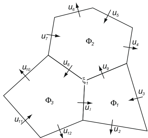
Fig. 3. Schematic showing the locations of the prognostic variables \Phi_i and u_e , as well as the natural location for diagnosing the relative vorticity \xi at vertex 1.
