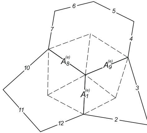
Fig. 5. Schematic showing the areas A_1^{(e)} , A_8^{(e)} , and A_9^{(e)} associated with edges 1, 9, and 8. The area associated with edge 1 comprises the two triangles either side of edge 1.
