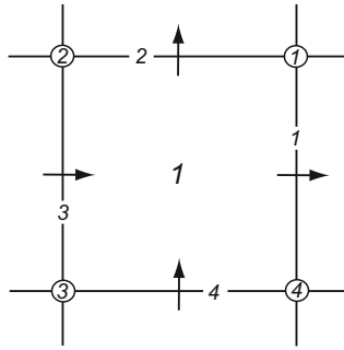
Fig. 6. Schematic showing the cell, edge and vertex numbering, and unit normal vectors at cell edges, for part of a square grid.
