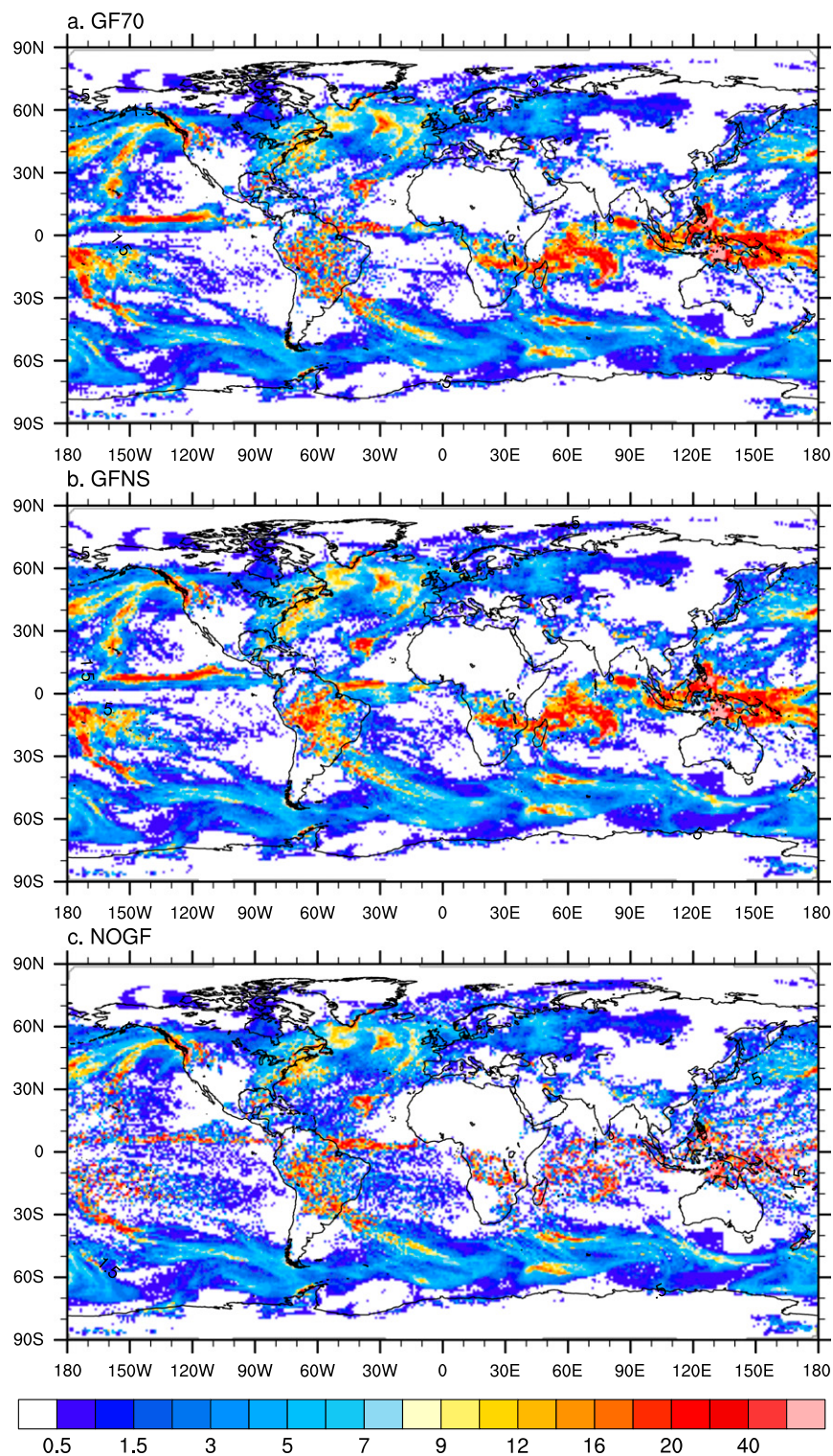
FIG. 8. As in Fig. 6, but for the total precipitation rate.
