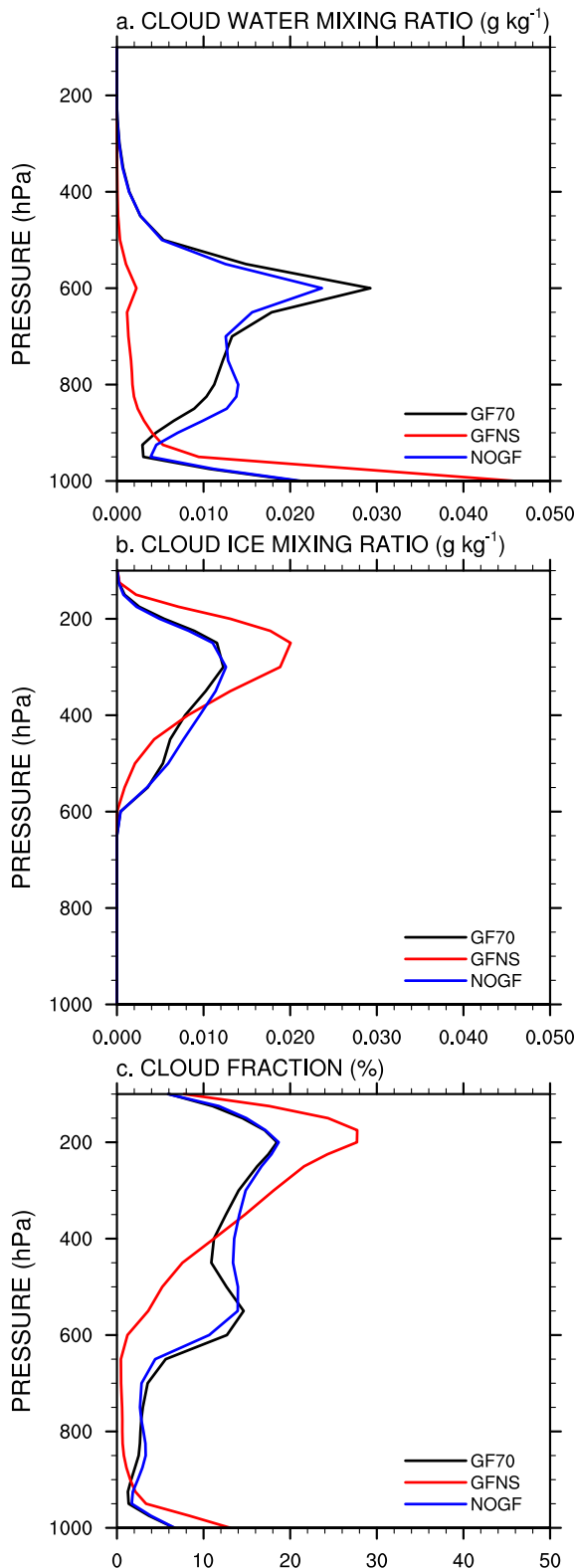
FIG. 12. Vertical distribution of the (a) cloud water mixing ratio ( \text{g kg}^{-1} ), (b) cloud ice mixing ratio ( \text{g kg}^{-1} ), and (c) grid-scale horizontal cloud fraction (%) simulated with GF70 (black line), GFNS (red line), and NOGF (blue line).
