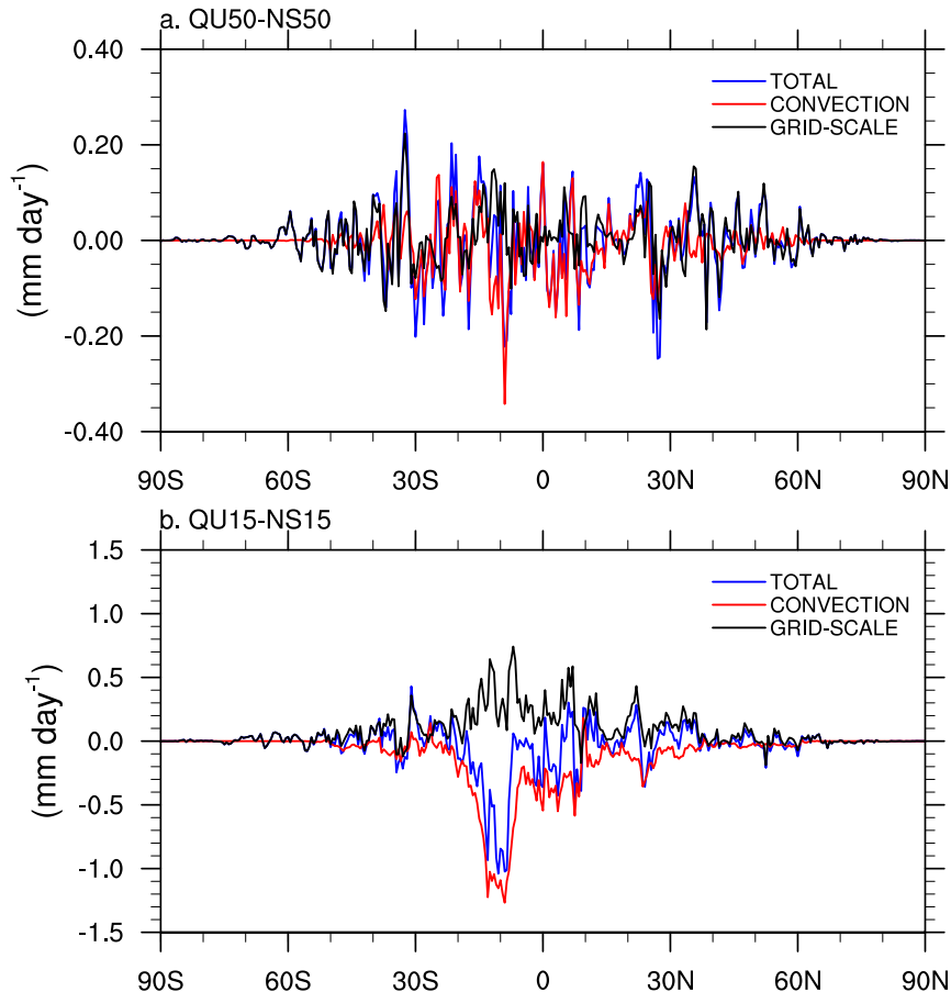
FIG. 5. Zonal mean differences in total, convective, and grid-scale precipitation rates calculated between 0000 UTC 11 Jan and 0000 UTC 14 Jan 2014: (a) QU50 minus NS50 and (b) QU15 minus NS15. Units are \text{mm day}^{-1} .
