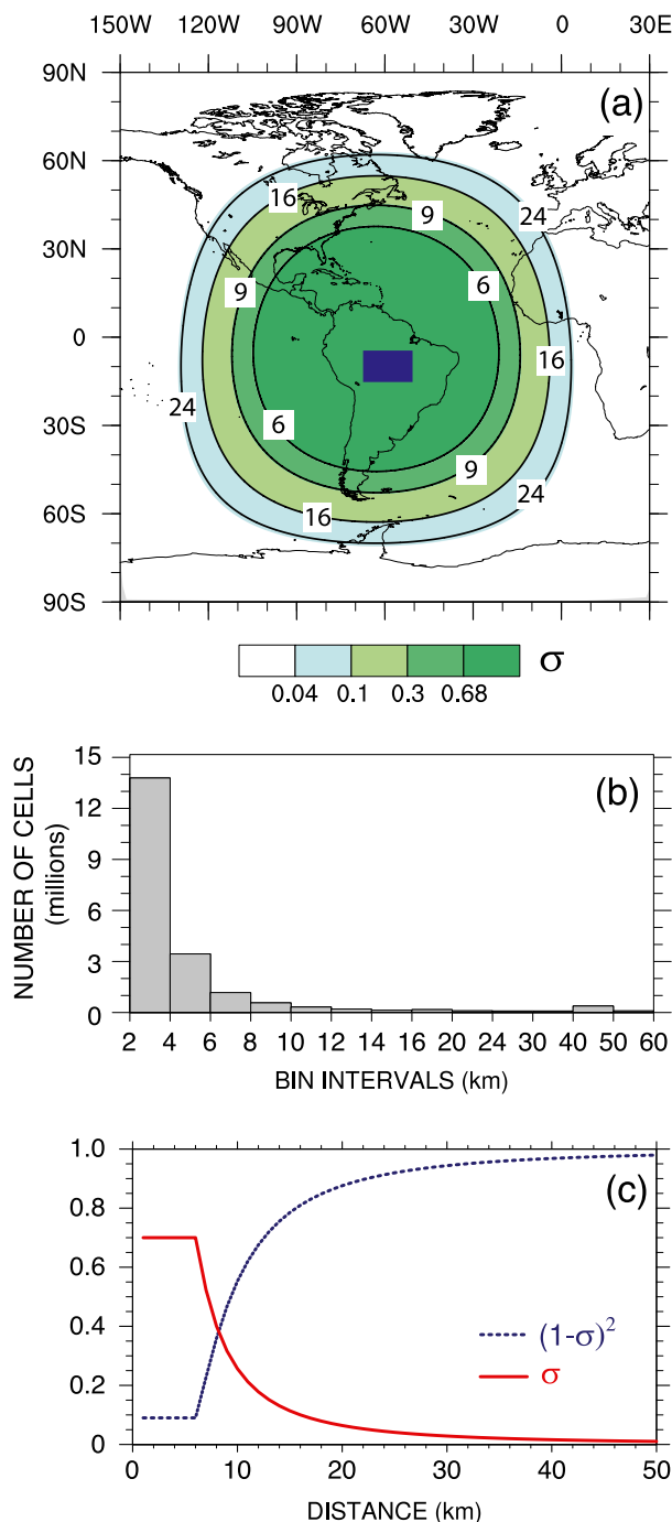
FIG. 1. (a) Refined area of the variable-resolution mesh over South America depicted using isolines of the mean distance between gridcell centers (km) and filled contours of the convective cloud fraction (dimensionless), (b) histogram of the number of grid cells as a function of the mean distance between gridcell centers, and (c) convective updraft fraction as a function of the mean distance between gridcell centers.
