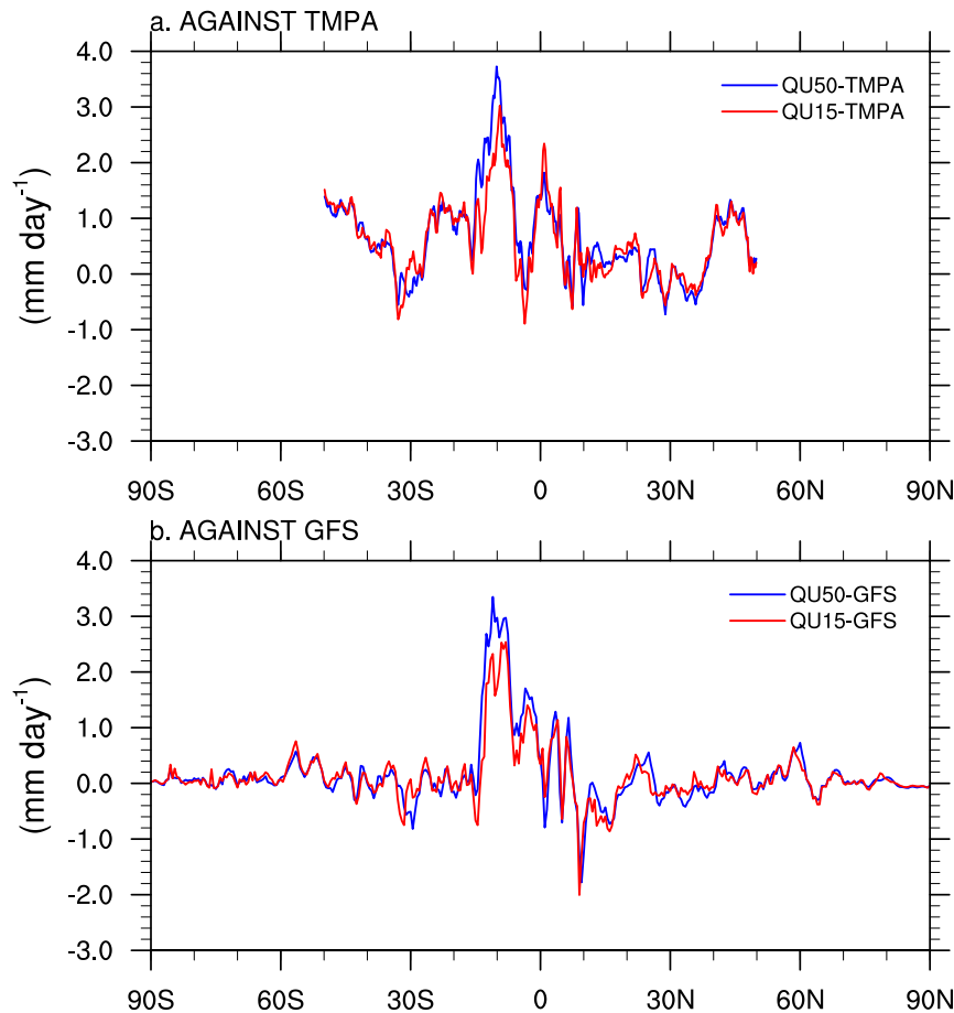
FIG. 3. Zonal mean differences in the precipitation rate calculated between 0000 UTC 11 Jan and 0000 UTC 14 Jan 2014 among (a) QU50, QU15, and TMPA data and (b) QU50, QU15, and GFS forecast. Units are \text{mm day}^{-1} .
