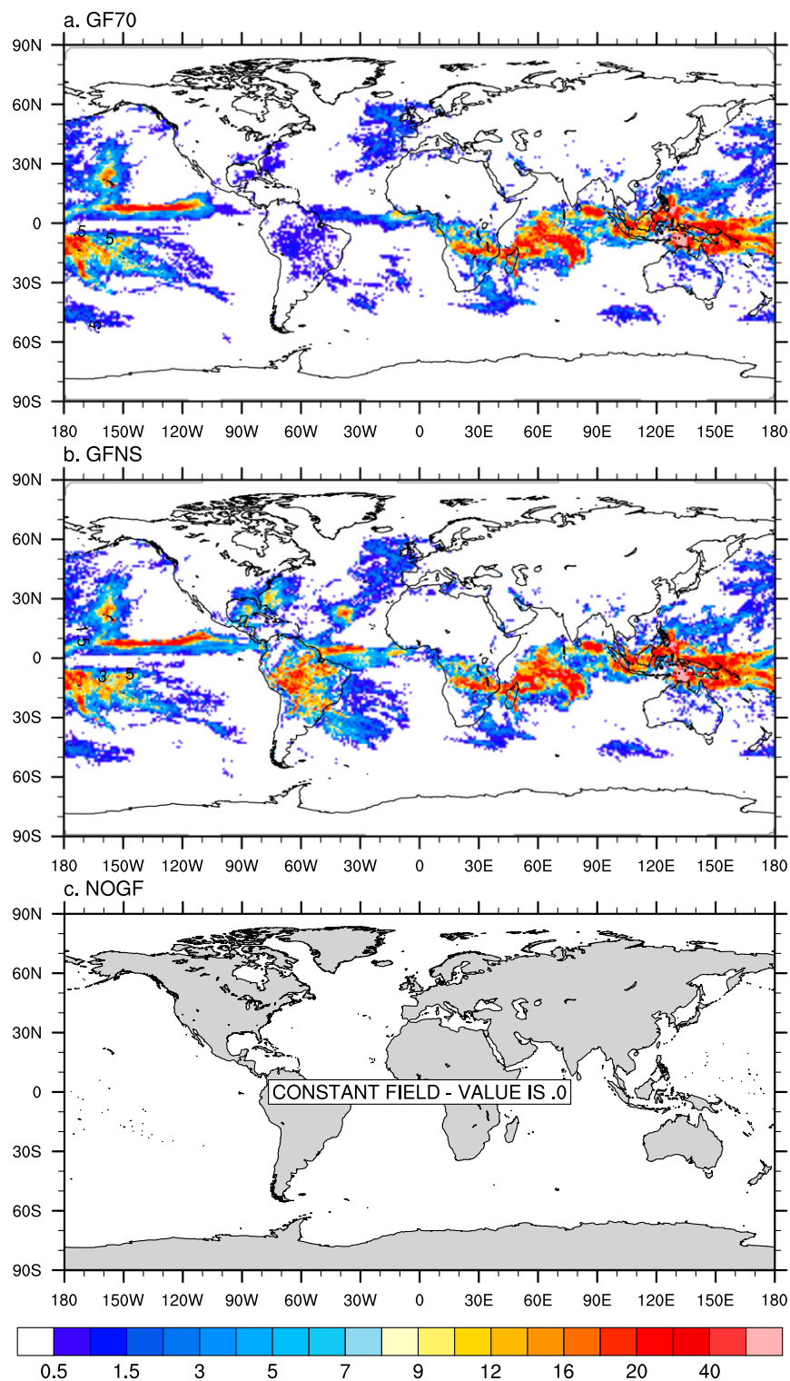
FIG. 6. Geographical distribution of the convective precipitation rate calculated between 0000 UTC 11 Jan and 0000 UTC 14 Jan 2014 and simulated with (a) GF70, (b) GFNS, and (c) NOGF. Units are \text{mm day}^{-1} .
