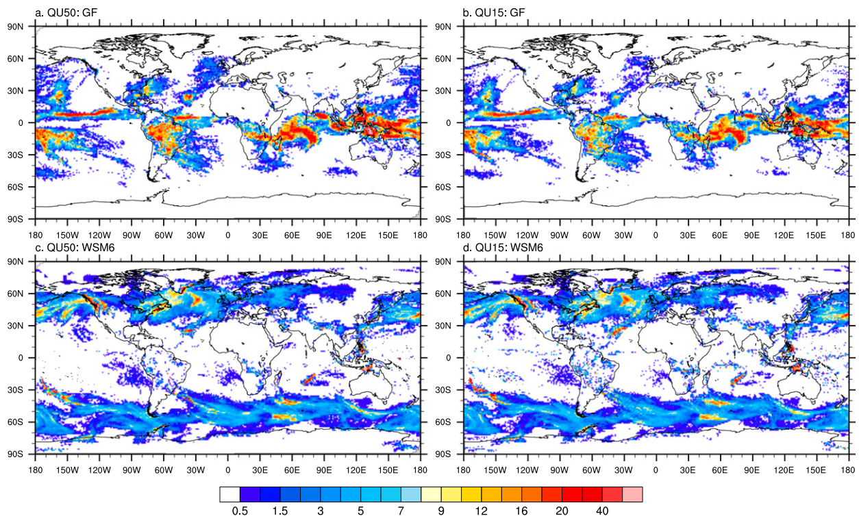
FIG. 4. Geographical distribution of the convective precipitation rate calculated between 0000 UTC 11 Jan and 0000 UTC 14 Jan 2014 and simulated with (a) QU50 and (b) QU15 and the grid-scale precipitation rate calculated between 0000 UTC 11 Jan and 0000 UTC 14 Jan 2014 and simulated with (c) QU50 and (d) QU15. Units are \text{mm day}^{-1} .
