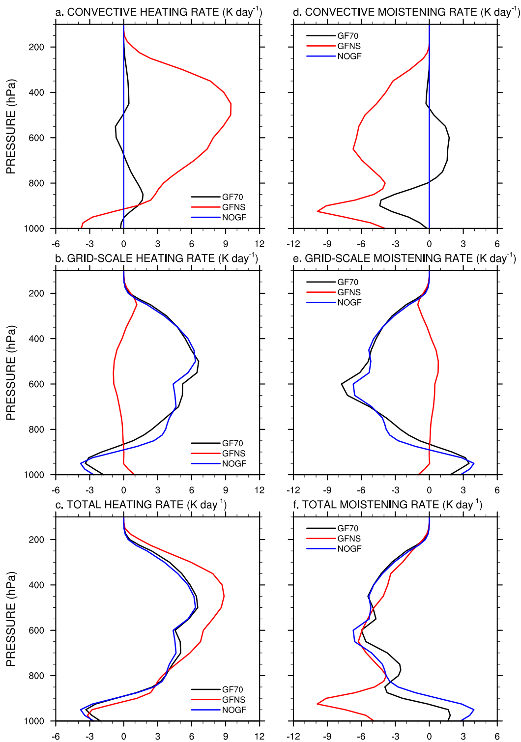
FIG. 11. (a)–(c) Vertical distribution of convective, grid-scale, and total heating rates and (d)–(f) convective, grid-scale, and total moistening rates simulated with GF70 (black line), GFNS (red line), and NOGF (blue line). Units are \text{K day}^{-1} .
