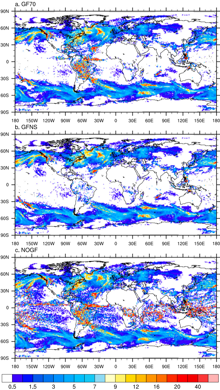
FIG. 7. As in Fig. 6, but for the grid-scale precipitation rate.
