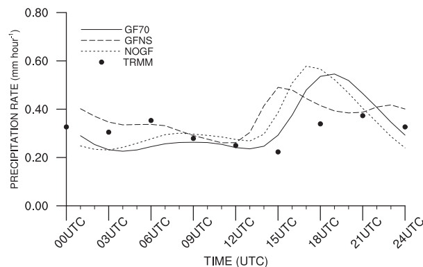
FIG. 10. Diurnal cycle of the precipitation rate simulated with GF70 (solid line), GFNS (dashed line), NOGF (dotted line), and TRMM data (dots). Units are \text{mm h}^{-1} .
