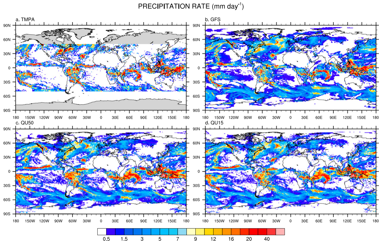
FIG. 2. Geographical distribution of the precipitation rate calculated between 0000 UTC 11 Jan and 0000 UTC 14 Jan 2014 obtained from (a) TMPA satellite data and (b) GFS forecast and simulated with (c) QU50 and (d) QU15. Units are \text{mm day}^{-1} .
