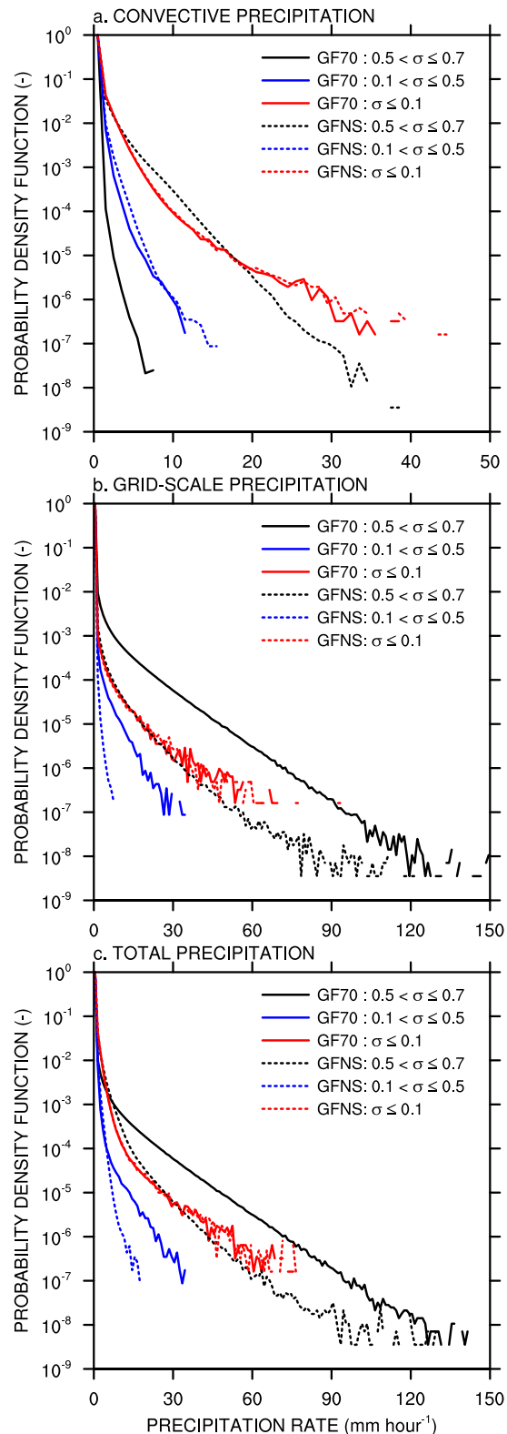
FIG. 9. Probability density distributions of the (a) convective precipitation rate, (b) grid-scale precipitation rate, and (c) total precipitation rate for GF70 (solid lines) and GFNS (dashed lines) as functions of the convective updraft fraction. Units are \text{mm h}^{-1} .
