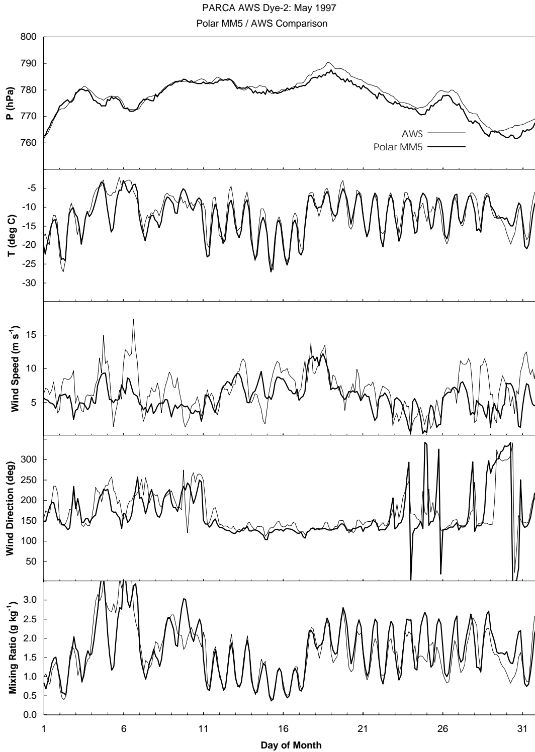
Figure 1. Time series plot of the AWS observed (thin solid line) and the Polar MM5 predicted (thick solid line) near surface air pressure (P), temperature (T), wind speed, wind direction, and water vapor mixing ratio at Dye-2, Greenland for May 1997. The model time series is a composite of the predictions valid 24-48 h after the model initial time.
