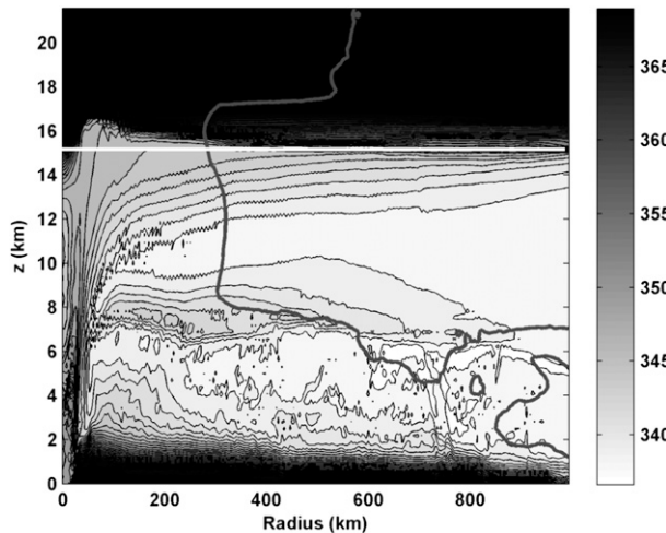
FIG. 3. Distribution in the radius–altitude plane of saturation equivalent potential temperature (K) averaged over the last 24 h of the numerical simulation described in the text. The thick gray curve represents the V = 0 contour and the thick white line represents the altitude of the ambient tropopause. For clarity, values of saturation equivalent potential temperature have been capped at 370 K.
