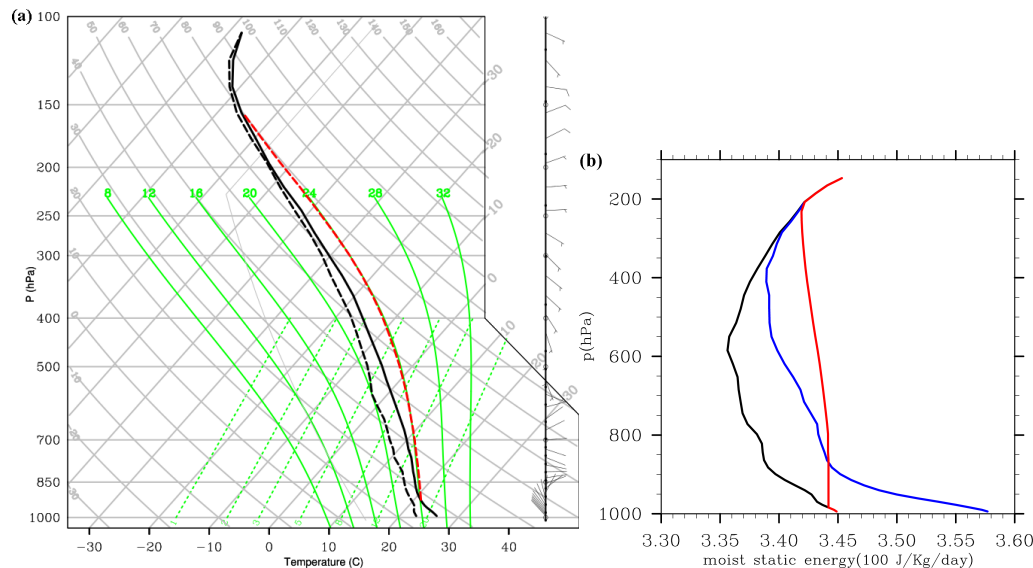
Fig. 2. Skewt diagram (a) displaying temperature (solid black line), dew point (dashed black line), vertical wind profile and the CAPE parcel profile (dashed red). Also shown are vertical profiles (b) of moist static energy (black), saturation moist static energy (blue) and simulated updraft moist static energy (red). Units for the abscissa.
