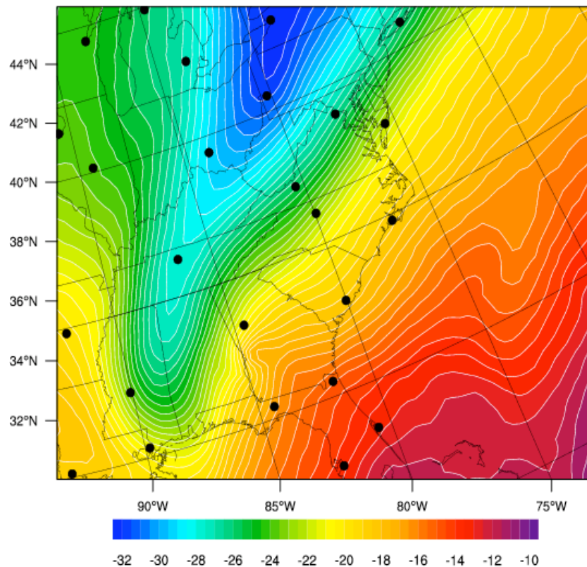
Temperature (C) at 500hPa
