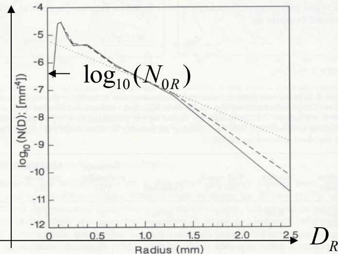
FIG. 9.21. Evolution of a drop spectrum in a subsaturated rainshaft including the effects of coalescence and breakup. The spectrum at the top of the rainshaft is Marshall-Palmer with a rainfall rate of 110 \text{ mm h}^{-1} . (.....), 0 km; (---), 1 km; (- - -), 2 km; R = 110 \text{ mm h}^{-1} ; t = 24 \text{ min} . From Tzivion et al. (1989). Journal of Atmospheric Sciences , 46, 21. American Meteorological Society. Reproduced with permission
