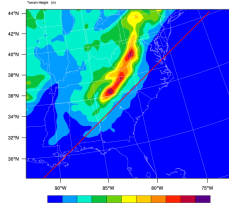
Terrain Height
