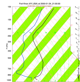
Skew-T Diagram
