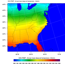
Soil Temperature
