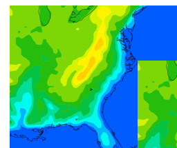
Domain Overlay
