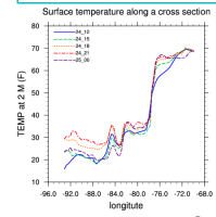
Sfc Temperature Horizontal X-section
