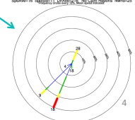
Wind Rose
