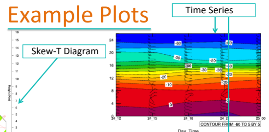
Time Series
