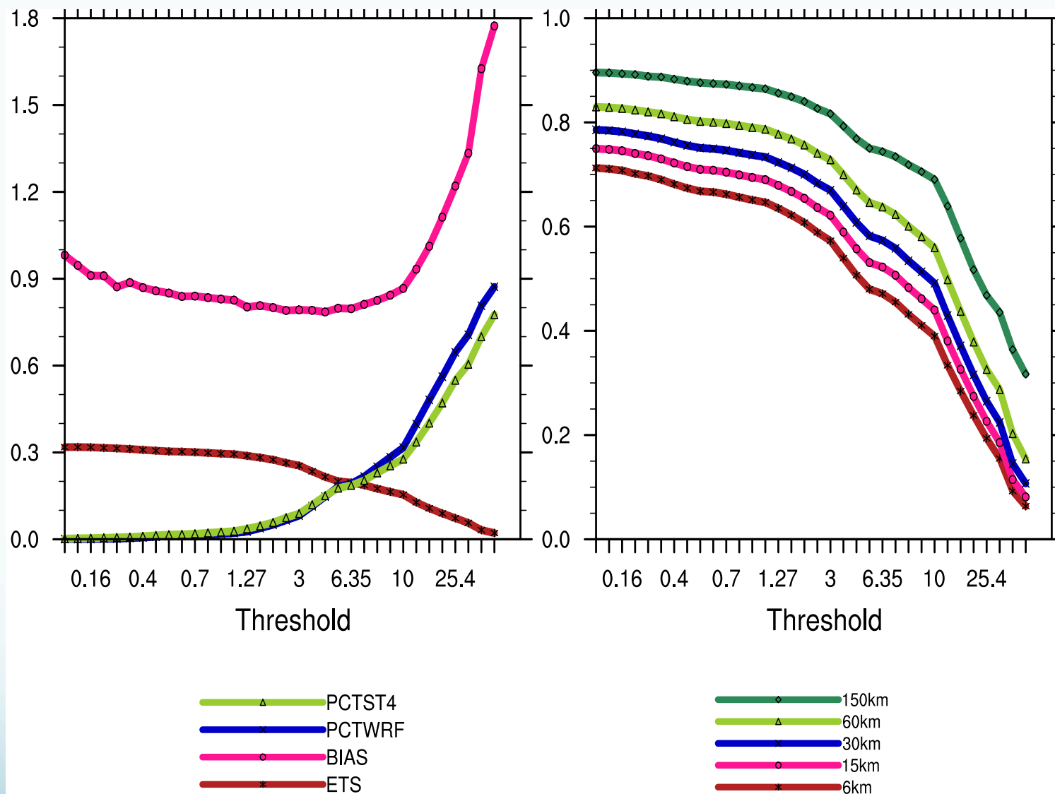
WRFV3.9, 3km Test Cases in Summer 2016
