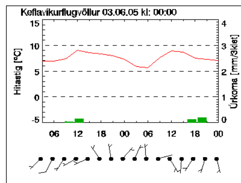
Figure 6: Forecasting diagram for Keflavík airport, SW-Iceland.
