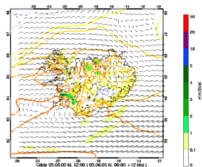
Figure 5: Accumulated 3 hours precipitation, two meter temperature and wind at 10 meters.
