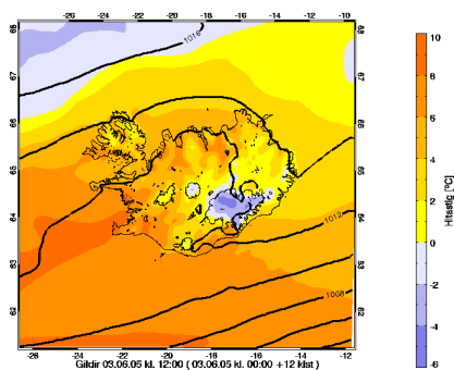
Figure 3: Temperature at two meter height.
