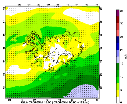
Figure 4: Windspeed and direction at 10 meters.
