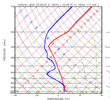
Figure 7: SkewT diagram for Keflavík airport, SW-Iceland.
