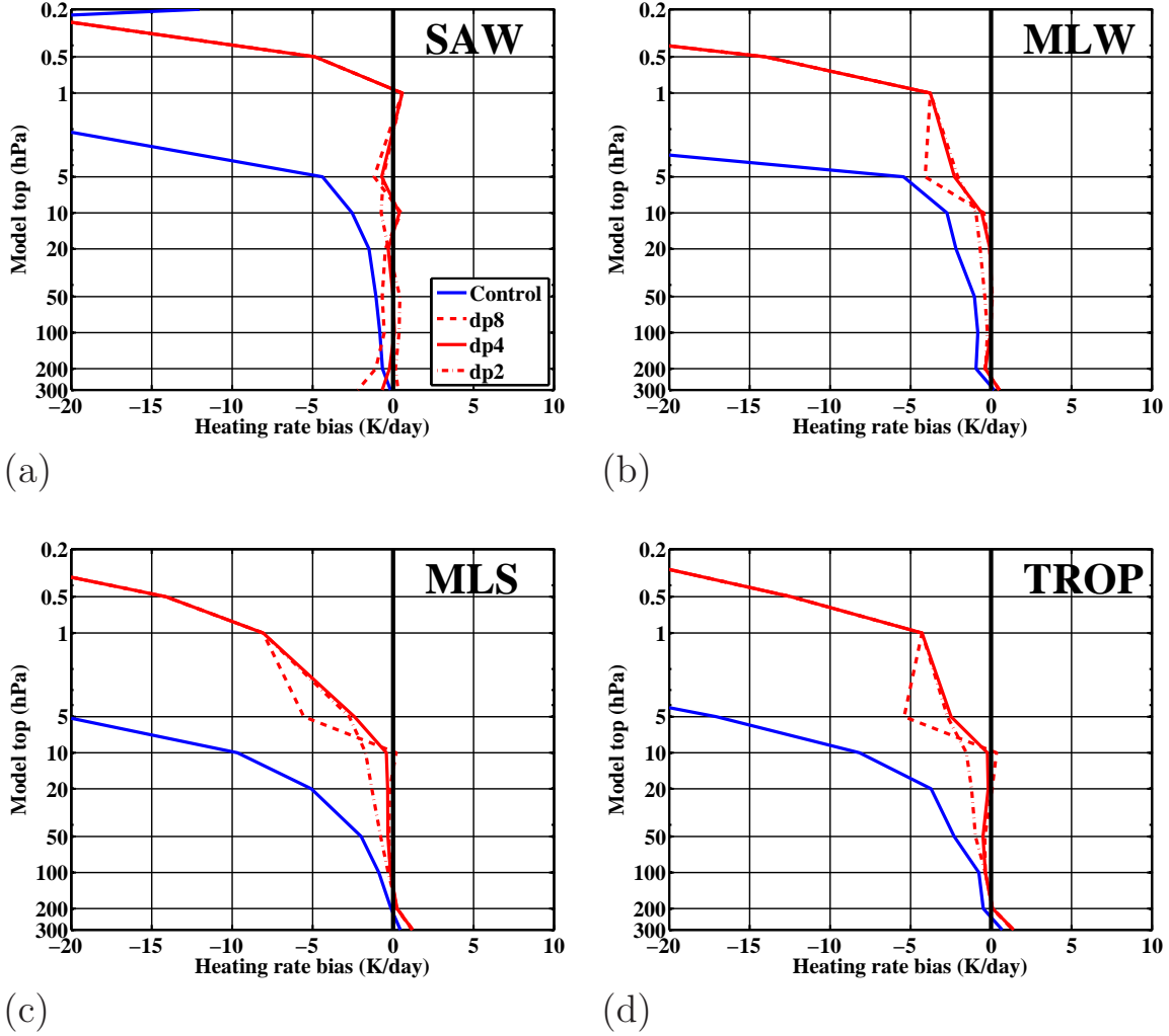
FIG. 3. Longwave radiative heating rates at the top model level minus the respective standard heating rate at the equivalent pressure level ( \dot{\theta}_{LW,model} - \dot{\theta}_{LW,standard} ) as a function of model top pressure based upon standard (a) subarctic winter (SAW), (b) midlatitude winter (MLW), (c) midlatitude summer (MLS), and (d) tropical (TROP) atmospheric vertical profiles. The difference in the control experiment is shown in blue. Experiments using a pressure interval of -8 hPa, -4 hPa, and -2 hPa between the model top and top of the atmosphere (TOA) are shown with the dashed, solid, and dashed-dot red contours respectively. Note the differences shown are not continuous profiles.
