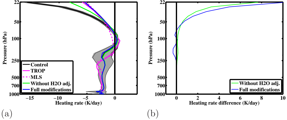
FIG. 5. Composite vertical longwave potential temperature (a) heating rates and (b) differences from the control case ( \dot{\theta}_{LW,experiment} - \dot{\theta}_{LW,control} ) of 6-hour forecasts initialized with GFS from 15 August 2009 at 00 UTC - 22 August 2009 at 00 UTC. The control case (no change in the RRTM longwave radiation scheme) is shown in black, while the standard tropical (TROP) and midlatitude summer (MLS) atmospheric profiles are shown by the magenta and magenta-dashed contours respectively. The experiment where only a buffer layer is added with \Delta p = -4\text{hPa} is shown in green, while the experiment with the buffer layer and adjustment to stratospheric water vapor are shown in blue. All profiles are averaged over the entire test domain (See Fig. 1a). In (a), the light (dark) gray shading represents the \pm 1 standard deviation limits of \theta_{LW} for the ‘Full modifications’ (‘Control’) experiments over the domain.
