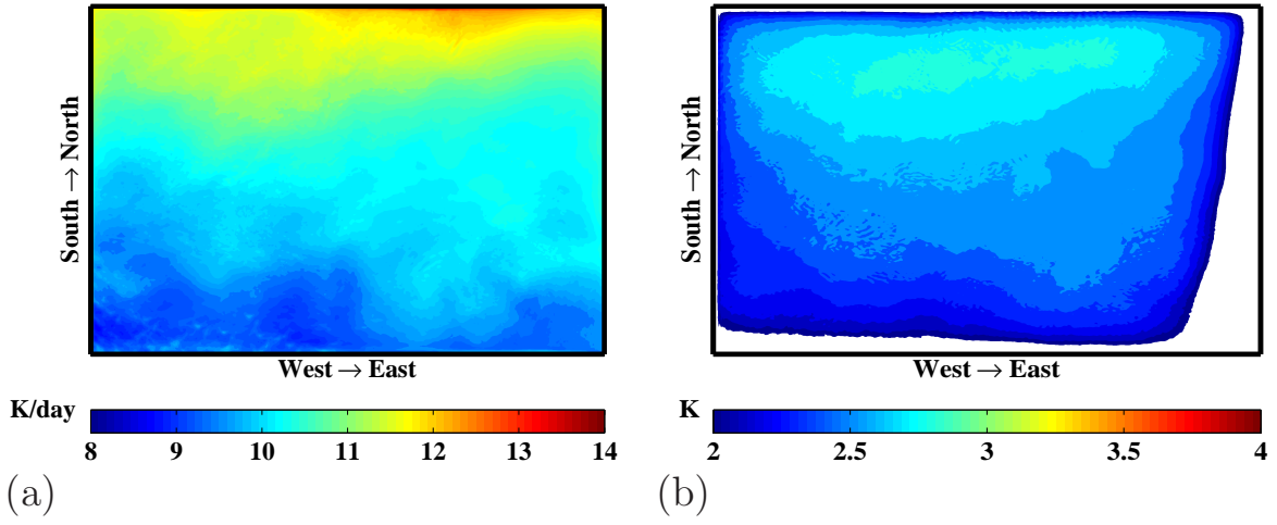
FIG. 6. Composite potential temperature (a) heating rate differences ( \dot{\theta}_{LW,experiment} - \dot{\theta}_{LW,control} ) and (b) changes in 6-hour forecasts of potential temperature ( \theta_{experiment,forecast} - \theta_{control,forecast} ) at the top model level between the control (no change in the RRTM longwave radiation scheme) and experiment (using the modified RRTM longwave radiation scheme). In (b), values below 2 K are shaded in white.
